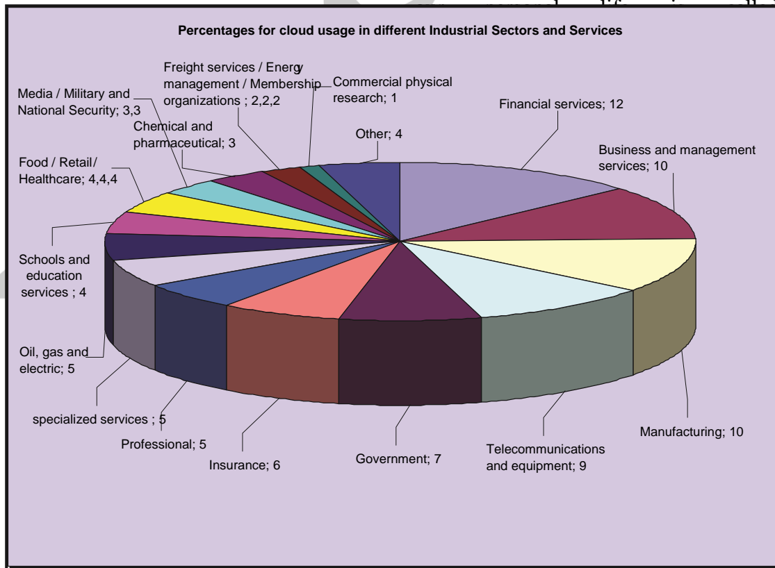
Figure 1. Cloud usage
