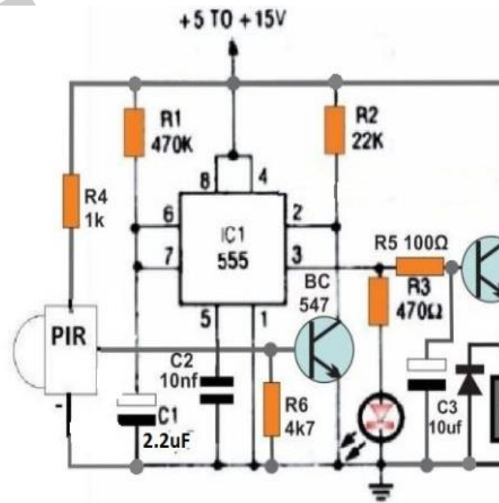
Fig 2.0: Circuit diagram of automatic hand sanitizer dispenser (Swagatam, 2020)
